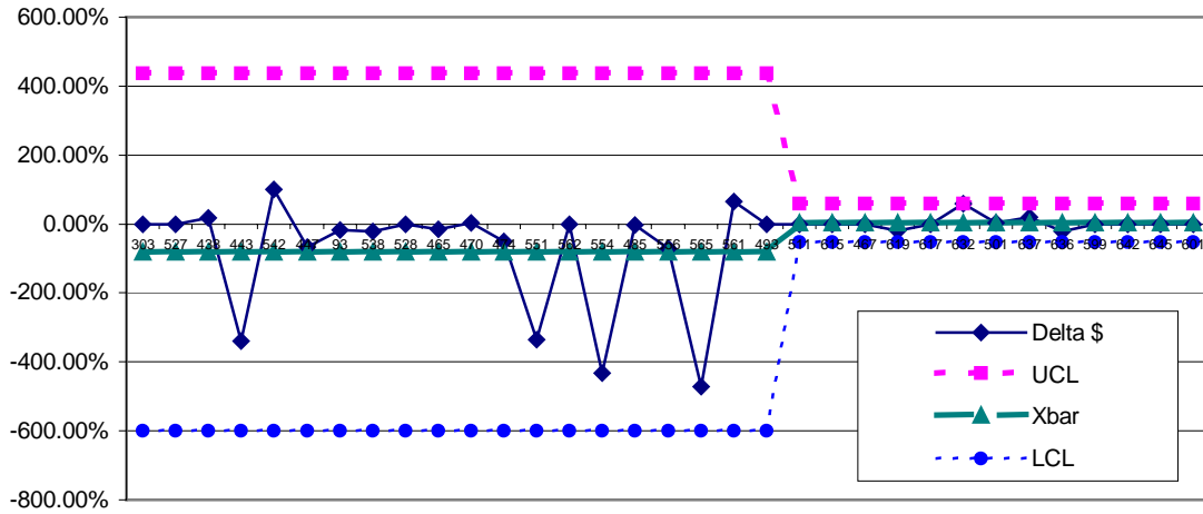
Delta $ (%) Control Chart
